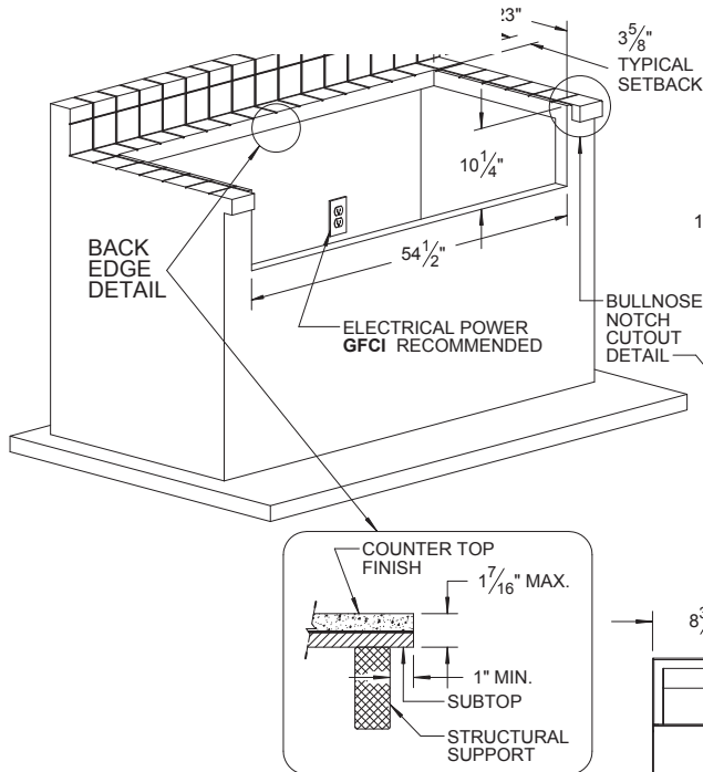
TYPICAL ALXE-56 BFG INSTALLATION
