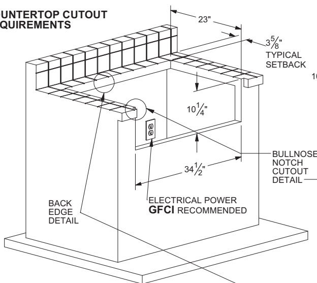
TYPICAL AIPG-36 INSTALLATION
