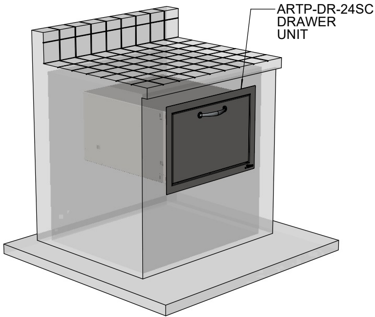
ARTP-DR-24SC DRAWER TYPICAL INSTALLATION
