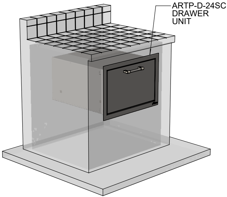
ARTP-D-24SC DRAWER TYPICAL INSTALLATION
