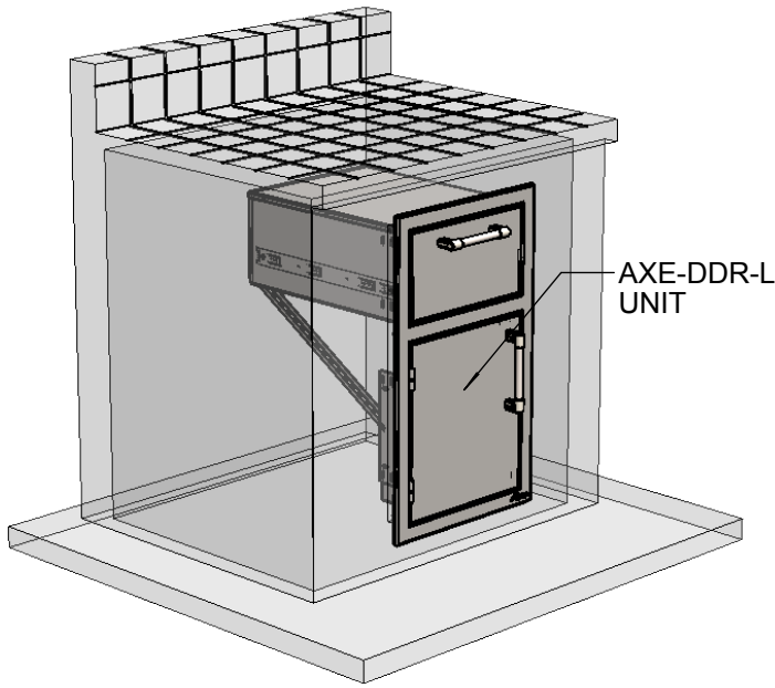
AXE-DDR-L TYPICAL INSTALLATION
