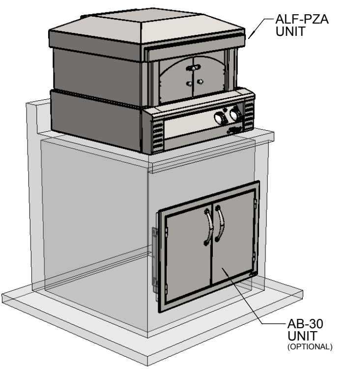
ALF-PZA TYPICAL COUNTER INSTALLATION
