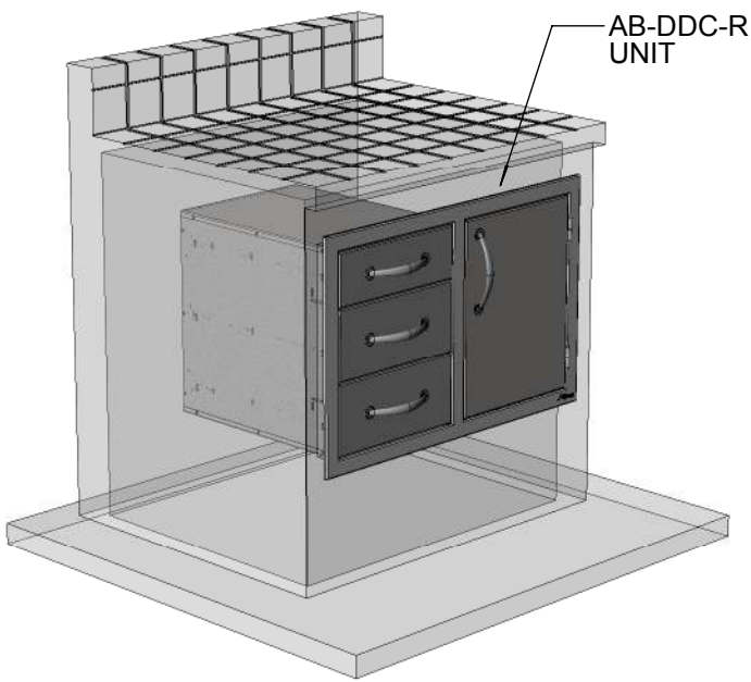
TYPICAL AB-DDC INSTALLATION
