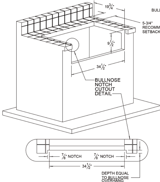
TYPICAL ART-36 INSTALLATION
