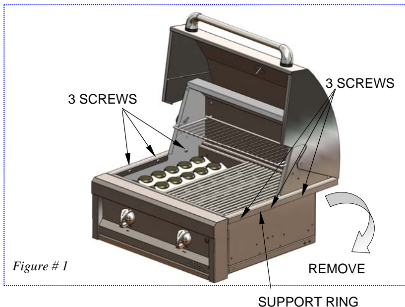
PERIMETER RING BRACKET
