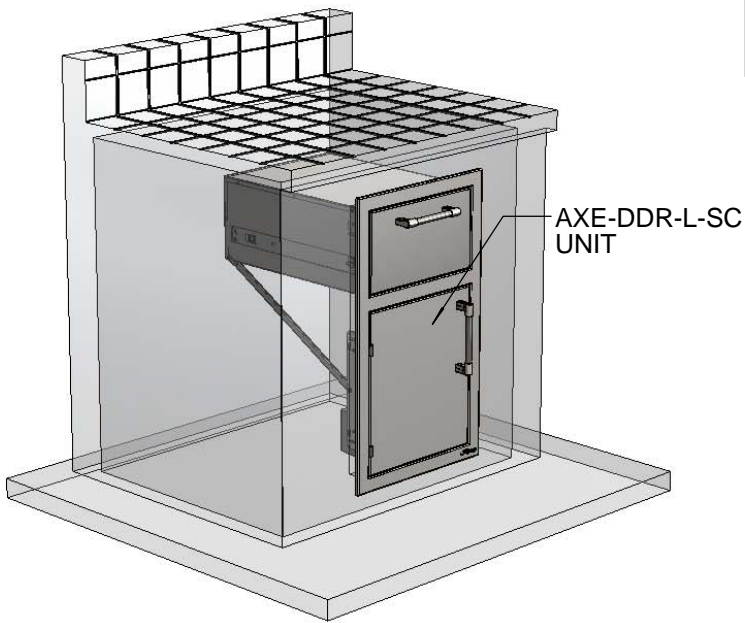
AXE-DDR-L-SC TYPICAL INSTALLATION
