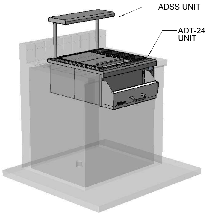
ADT-24 TYPICAL INSTALLATION (SHOWN WITH OPTIONAL ADSS SERVING SHELF)
