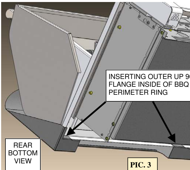
LIFT BBQ FROM ONE SIDE AT A TIME AND PLACE WIND SHIELD UNDER THE BBQ PERIMETER RING
