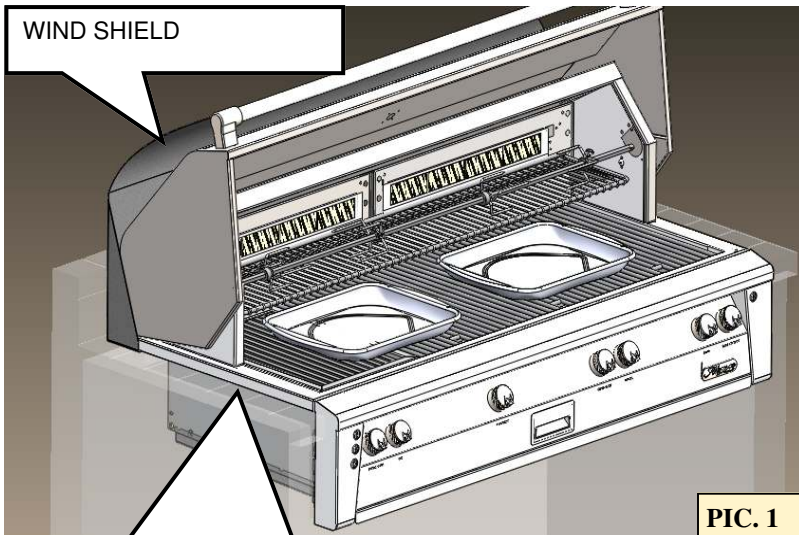
LIFT BBQ FROM ONE SIDE AT A TIME AND PLACE WIND SHIELD UNDER THE BBQ PERIMETER RING
