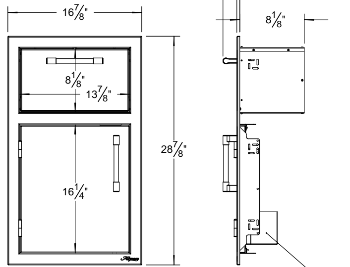
XEDS-4 DOOR ACCESSORY BOX (sold separately)
