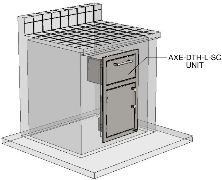
AXE-DTH-L-SC TYPICAL INSTALLATION
